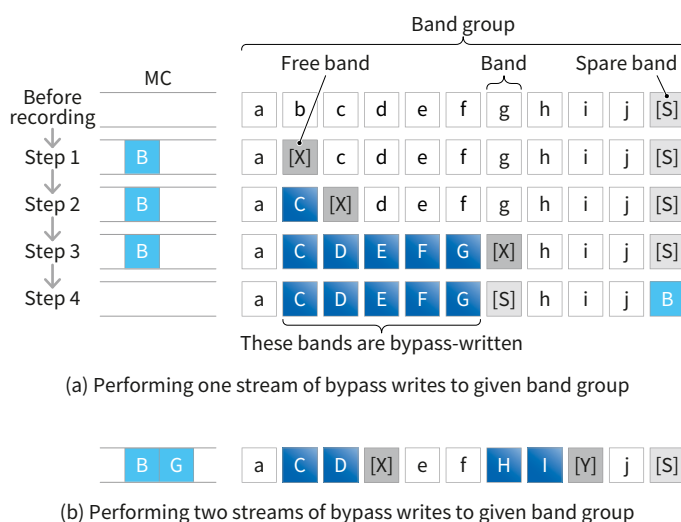
Figure 4. Bypass writing operations in band group using free bands – Free bands are generated when data are written to the MC. Bypass writes are performed using free bands.
